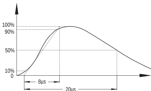
Curve 8/20 \mu s
